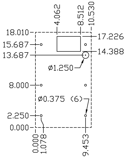
IQ150FPW INTAKE CUT OUT DRAWING
