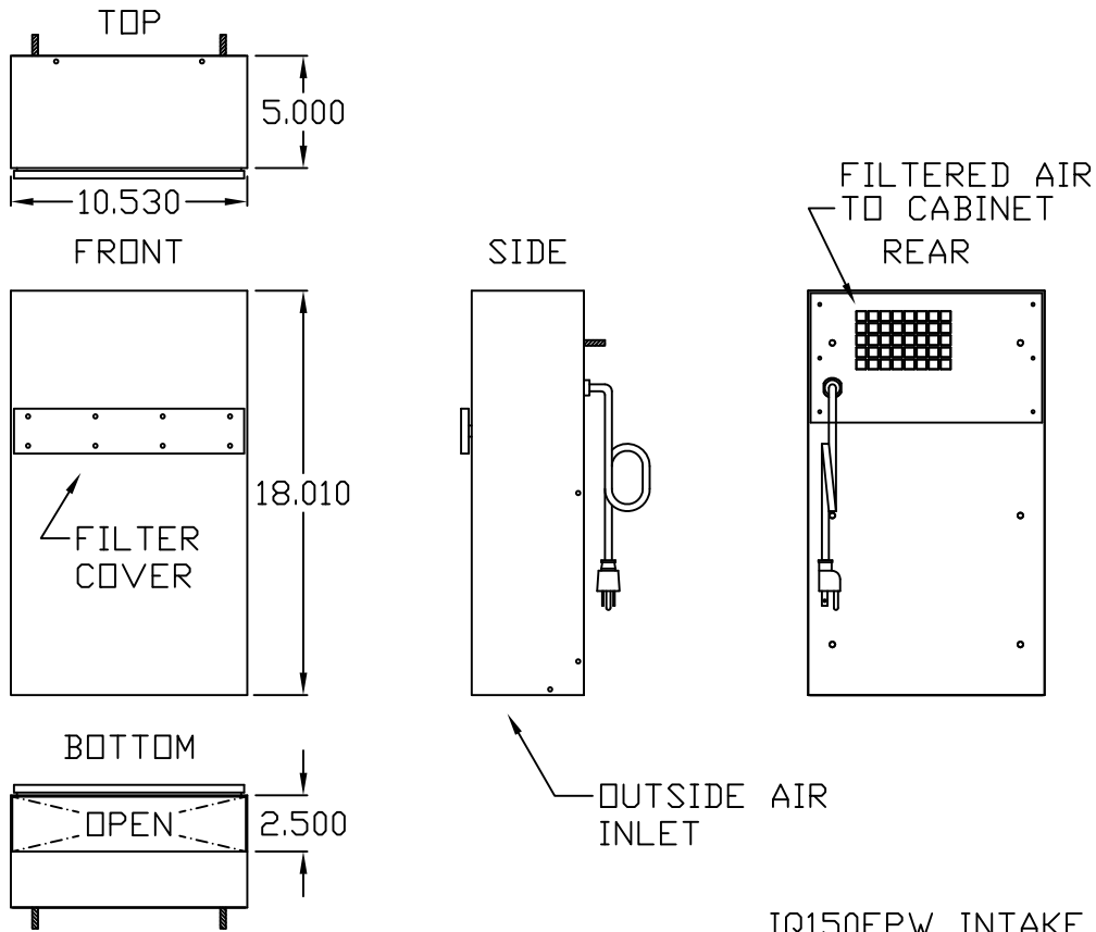
IQ150FPW INTAKE CUT OUT DRAWING
