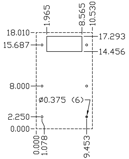
IQ150FPW EXHAUST CUT OUT DRAWING
