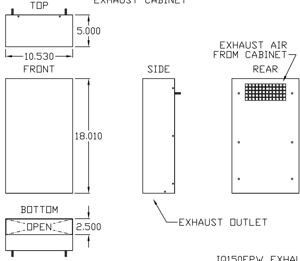
IQ150FPW EXHAUST CUT OUT DRAWING
